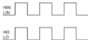
Figure 1. Input/Output Timing Diagram
