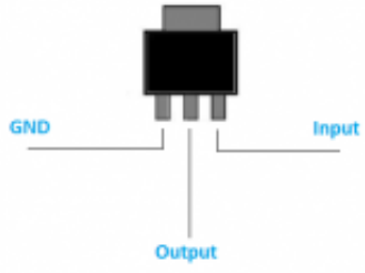
AMS1117 Pinout
