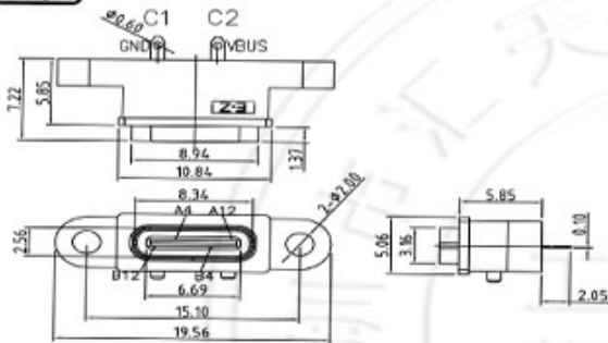
PIN ASSIGNMENT
